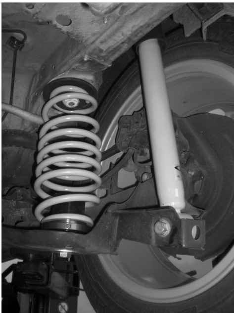
V7 Verbundlenker-Hinterachse twist-beam rear axle
